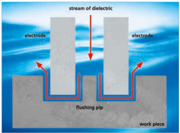
Figure 2: Pressure flushing
