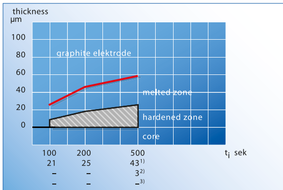
Figure 6a: Thickness of layers and amount of cracks in the rim after spark erosion on hardened (52 HRC) UHB Ovrar 2 microdized at different lengths of firing period
