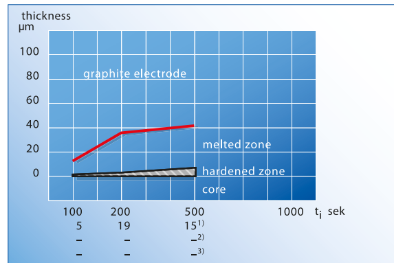
Figure 6b: The same after spark erosion on UHB Ovrar 2 microdized which has been annealed
