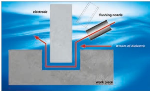
Figure 1: Open flushing
